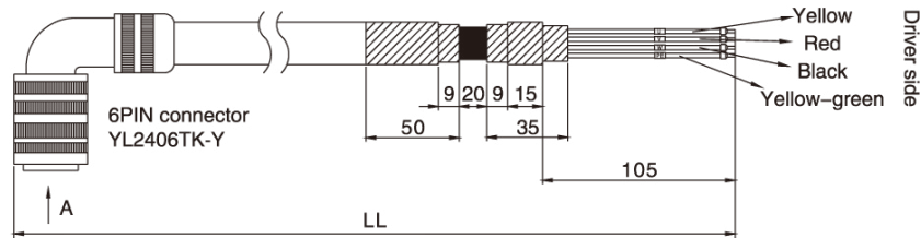
Motor Cable: MOT-008-05-KC2 for SMH150D-0230/0300/0380
