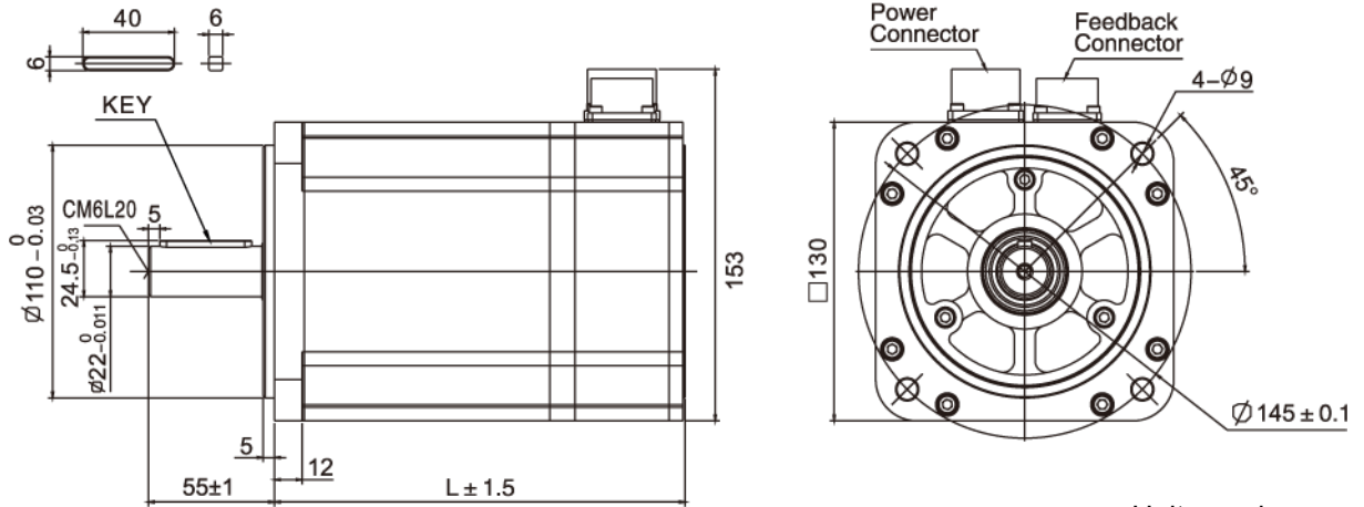
SMH130D Dimension Drawing
