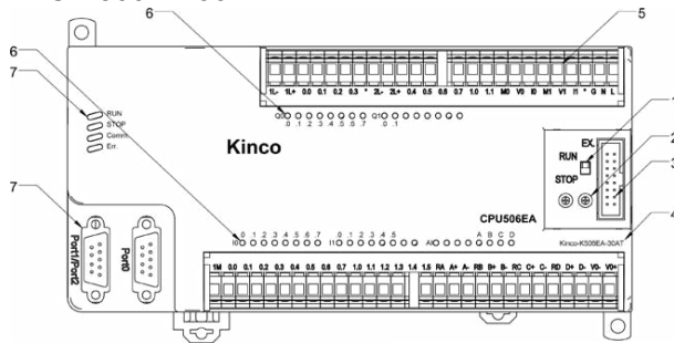
PLC-K506EA-30AT
