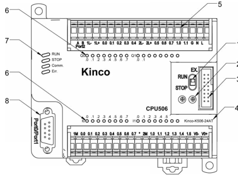
PLC-K506-24AT
