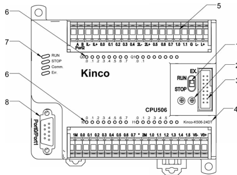
PLC-K506-24DT
