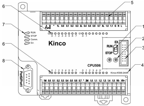
PLC-K506-24AR
