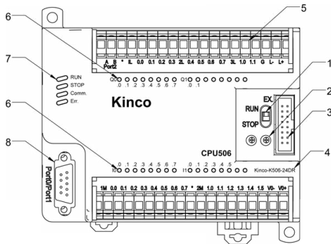
PLC-K506-24DR
