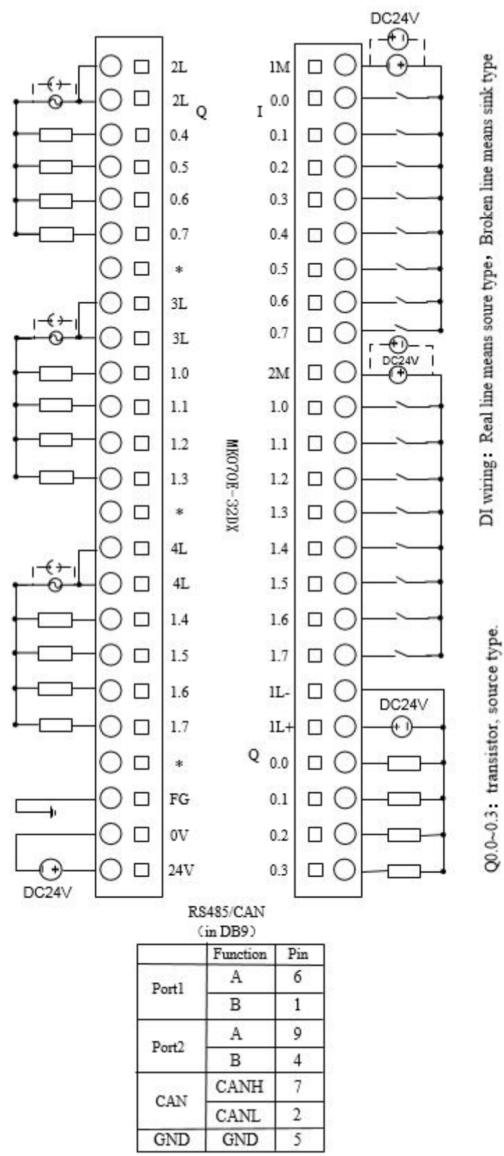
MK070E-32DX wiring diagram
