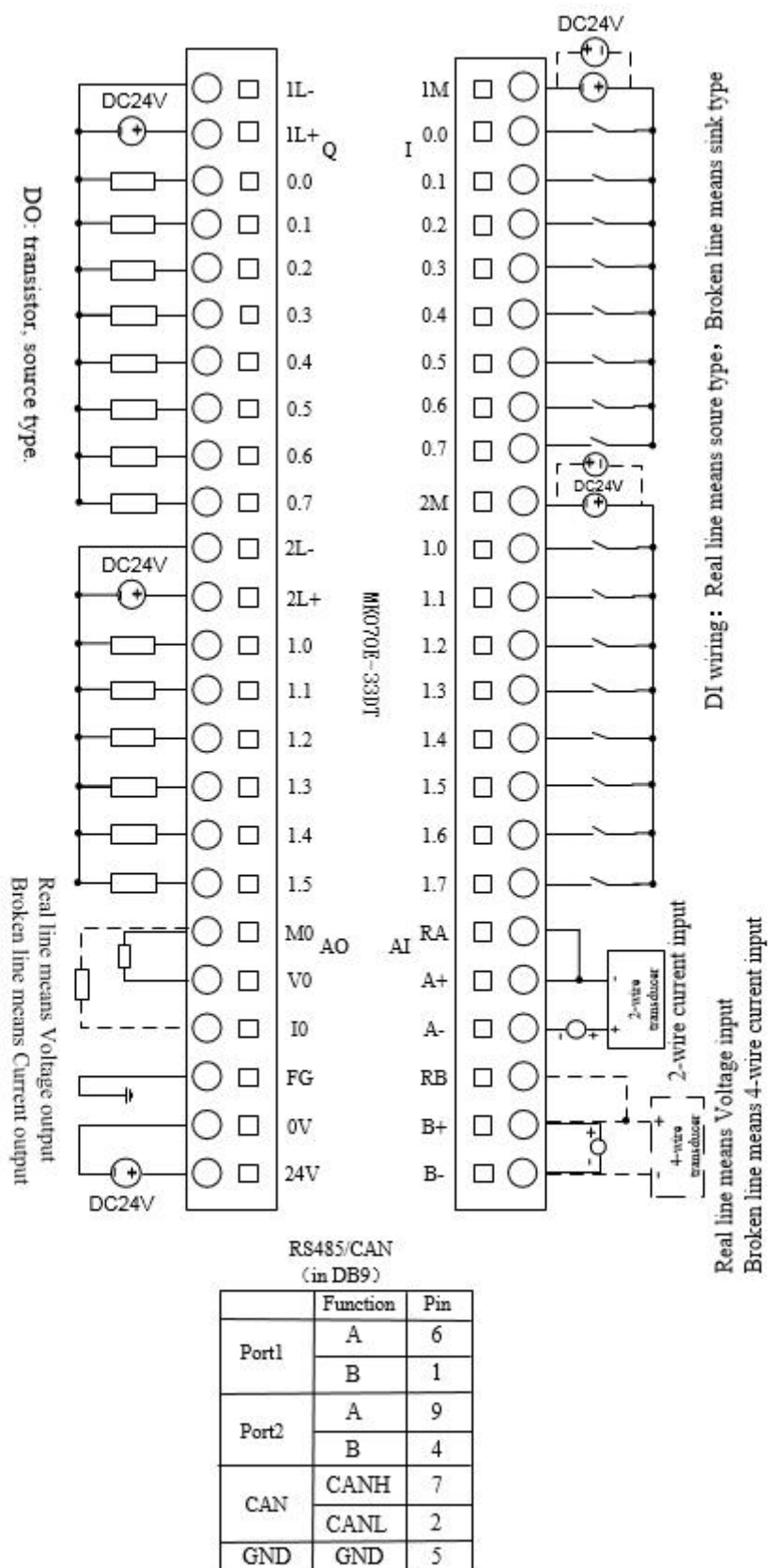
MK070E-33DT wiring diagram
